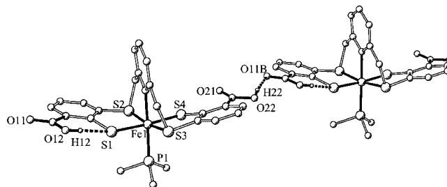
Figure 5. Intra- and intermolecular hydrogen bonds of [\text{Fe}(\text{PMe}_3)(\text{pyCO}_2\text{HS}_4)] ( 12 )
