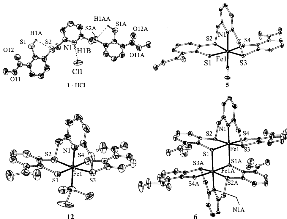
Figure 4. Molecular structures of \text{pyCO}_2\text{MeS}_4\text{-H}_2\text{-HCl} ( 1 ·HCl), [\text{Fe}(\text{CO})(\text{pyCO}_2\text{MeS}_4)] ( 5 ), [\text{Fe}(\text{pyCO}_2\text{MeS}_4)]_2\text{-H}_2\text{O-THF} ( 6 ·H 2 O·THF) and [\text{Fe}(\text{PMe}_3)(\text{pyCO}_2\text{HS}_4)]\cdot 0.25\text{MeOH} ( 12 ·0.25MeOH) (50% probability ellipsoids, C-bonded H atoms and solvent molecules omitted)
