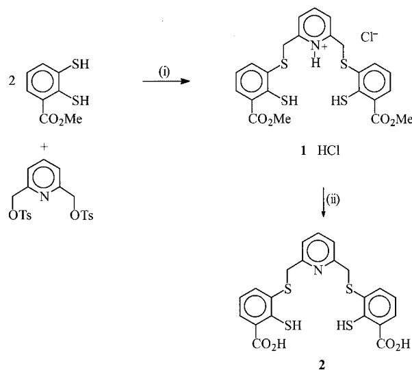
Scheme 1. Synthesis of the target ligands 1 and 2 : (i) 1) +2 \text{NMe}_4\text{OH} , -78^\circ\text{C} , THF/MeOH, 15 h; 2) \text{HCl}_{\text{aq.}} , \text{CH}_2\text{Cl}_2 ; 3) +2 \text{LiOMe} , + \text{Ni}(\text{OAc})_2\cdot 4\text{H}_2\text{O} , MeOH; 4) \text{HCl}_{\text{aq.}} , \text{CH}_2\text{Cl}_2 . (ii) 1) +10 \text{NaOH}_{\text{aq.}} , THF, 72 h; 2) \text{HCl}_{\text{aq.}} , \text{CH}_2\text{Cl}_2
