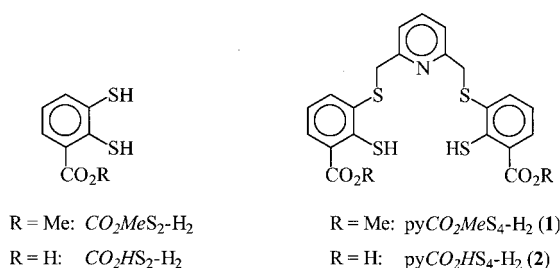
Figure 2. Starting materials, notations and the target ligands 1 and 2
