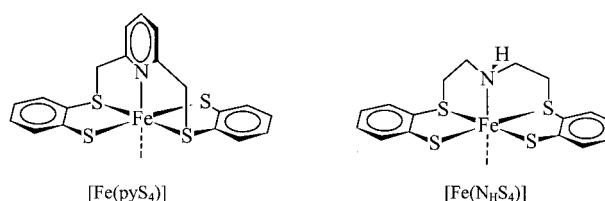
Figure 1. Schematic structure of [Fe(pyS 4 )] and [Fe(N H S 4 )] fragments
