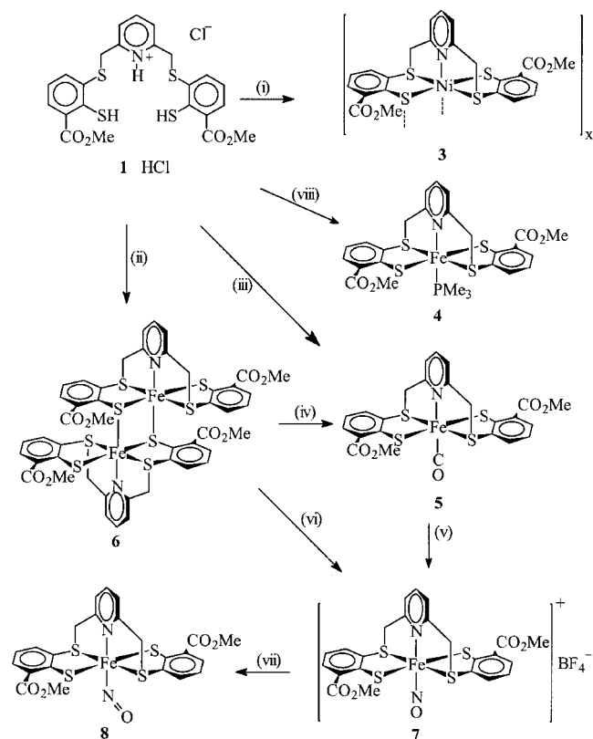
Scheme 2. Fe and Ni complexes with [\text{M}(\text{pyCO}_2\text{MeS}_4)] fragments: (i) + 3 LiOMe, + \text{Ni}(\text{OAc})_2 \cdot 4\text{H}_2\text{O} , MeOH; (ii) + 3 LiOMe, + \text{FeCl}_2 \cdot 4\text{H}_2\text{O} , MeOH; (iii) + 3 LiOMe, + \text{FeCl}_2 \cdot 4\text{H}_2\text{O} , + exc. CO, MeOH; (iv) + exc. CO, THF; (v) + \text{NOBF}_4 , \text{CH}_2\text{Cl}_2 ; (vi) + 2 \text{NOBF}_4 , \text{CH}_2\text{Cl}_2 ; (vii) + exc. \text{H}_2\text{N}_4 , MeOH; (viii) + 3 LiOMe, + \text{FeCl}_2 \cdot 4\text{H}_2\text{O} , + exc. \text{PMe}_3 , MeOH
