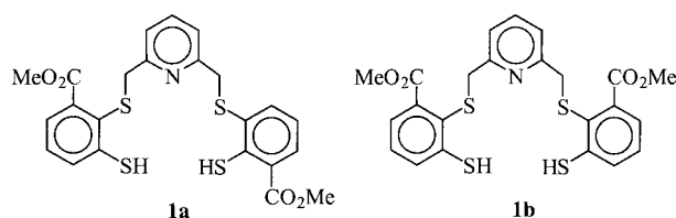
Figure 3. Isomers of \text{pyCO}_2\text{MeS}_4\text{-H}_2 ( 1 )
