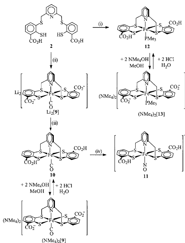
Scheme 3. Synthesis of acidic [\text{Fe}(\text{L})(\text{pyCO}_2\text{HS}_4)] complexes and corresponding salts with [\text{Fe}(\text{L})(\text{pyCO}_2\text{S}_4)]^{2-} anions: (i) + \text{FeCl}_2 \cdot 4\text{H}_2\text{O} , + exc. \text{PMe}_3 , MeOH; (ii) + 4 LiOMe, + \text{FeCl}_2 \cdot 4\text{H}_2\text{O} , + exc. CO, MeOH; (iii) + 2 HCl, \text{H}_2\text{O} (iv) + \text{NOBF}_4 , \text{CH}_2\text{Cl}_2
